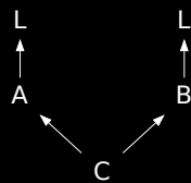
Figure 3: Non-virtual base [fig:class.nonvirt]
