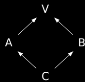
Figure 4: Virtual base [fig:class.virt]
